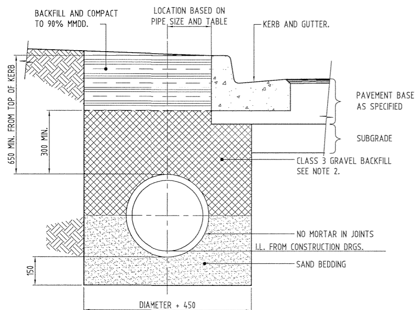
NORMAL DETAIL (375 - 825 DIA.)
