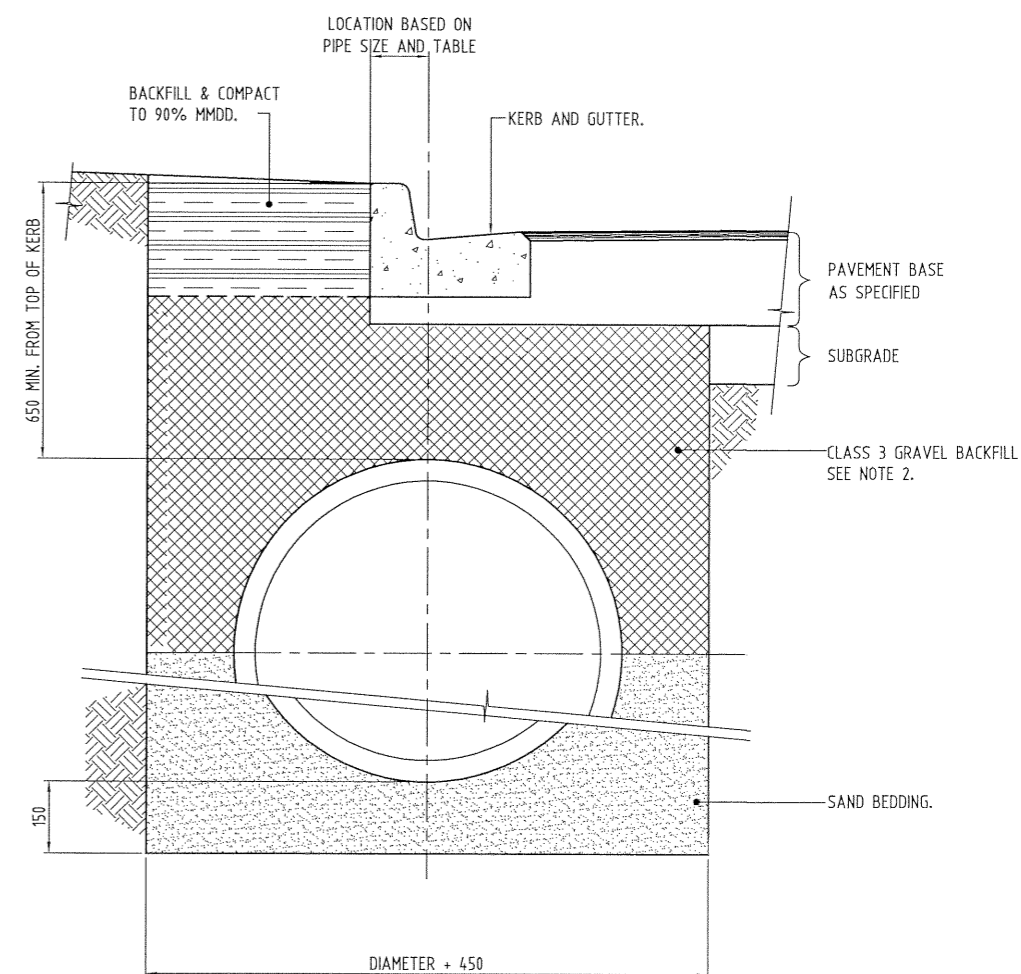
LARGE PIPE DETAIL (900 DIA UPWARDS)
