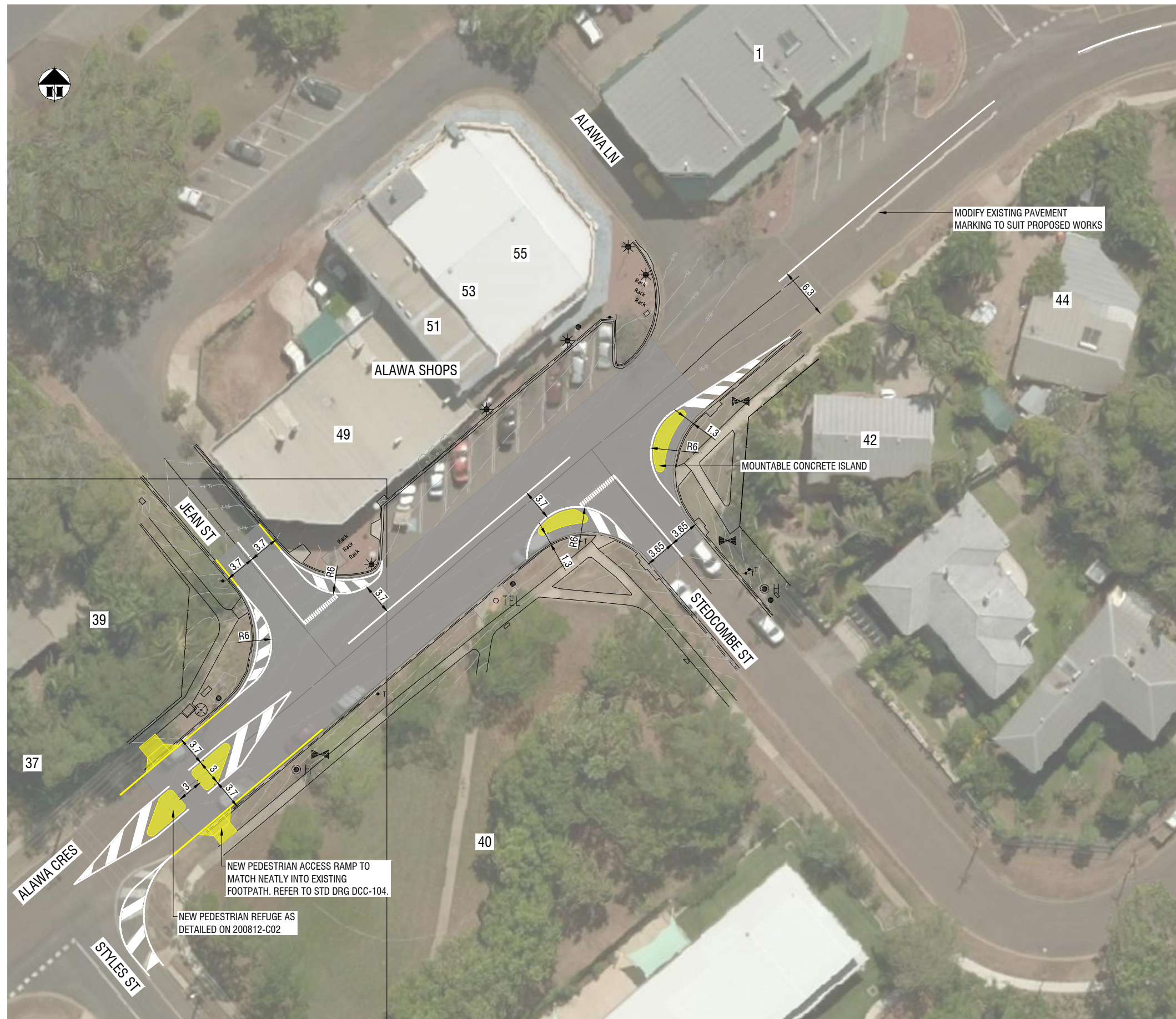
SITE 3 - ALAWA CR - JEAN & STEDCOMBE ST INTERSECTIONS SCALE: 1:250 @ A1
